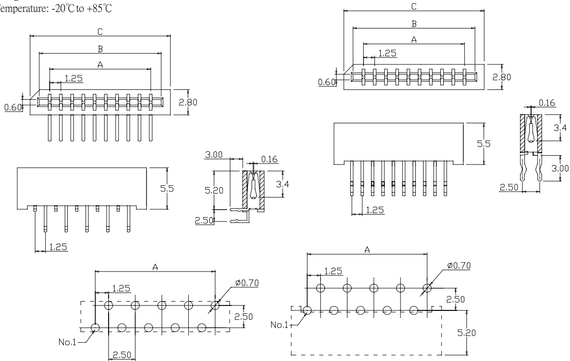
Recommended PCB Layout (PCB TOLERANCE±0.05)
